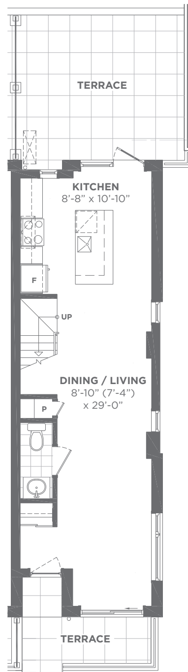
Ground Floor
